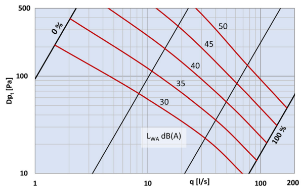
Diagram 3: Total A-weighted sound power level, dB(A) for SPMF-160
