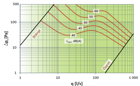
Diagram 6: Ljuddiagram SPMF-315
